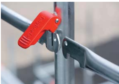
Guard rail bracket indicates unsecured guard rails
